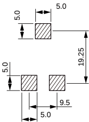
Land Pattern: [mm]
