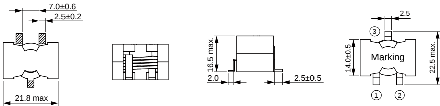
Dimensions: [mm]
