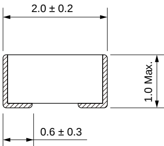
Dimensions: [mm]
