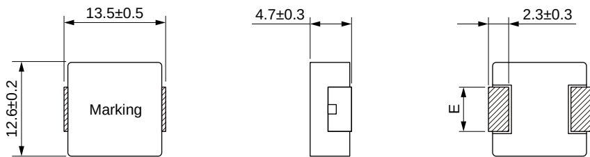
Dimensions: [mm]
