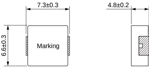
Dimensions: [mm]
