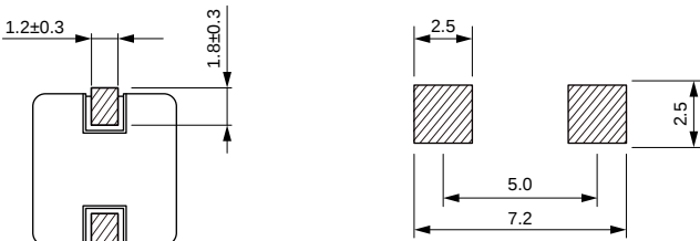
Land Pattern: [mm]
