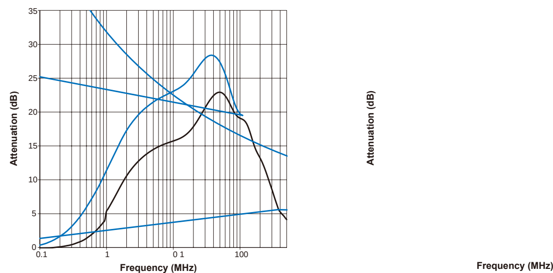
Insertion Loss Common Mode
